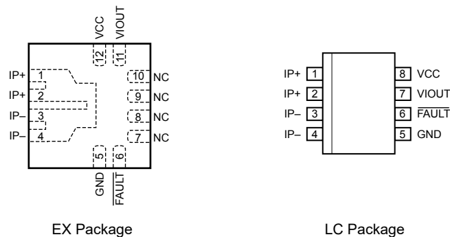
PINOUT DIAGRAMS
