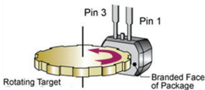
Figure 6: Left-to-Right, Pin 1 to Pin 3 Direction of Target Rotation.
